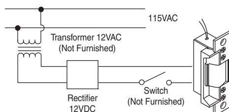
Typical Wiring Diagram AC Power Source – Silent Operation
