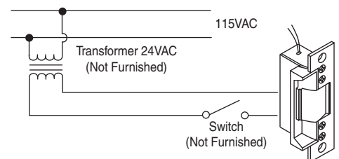
Typical Wiring Diagram AC Power Source – Audible Operation
