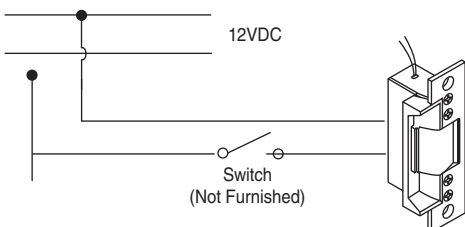
Typical Wiring Diagram DC Power Source – Silent Operation
